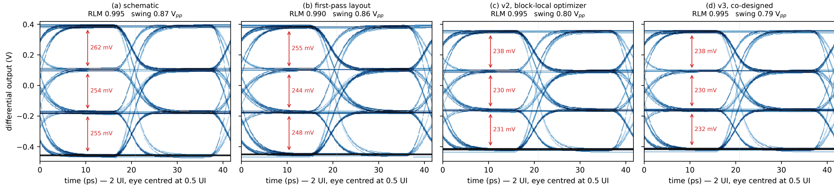
48 GBd PAM-4 eye — 200 mV pp input, 4 ps edges, seed-7 MSB/LSB streams; post-layout tiers on the kpex 2.5D CC extraction
