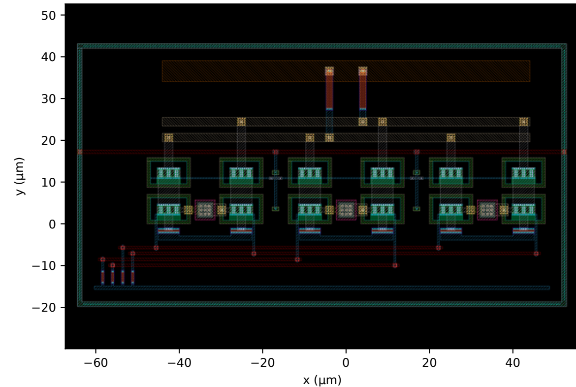
(b) first-pass layout (v1 floorplan, nominal sizing) 117.2 \times 62.9 \mu\text{m} = 7374 \mu\text{m}^2 S11 -8.90 / S22 -7.97 dB 191 mW
