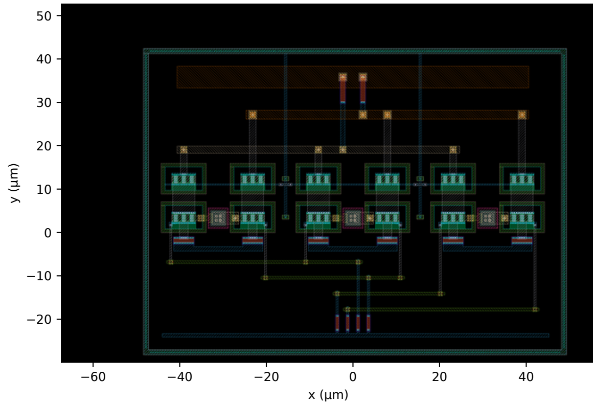
(d) co-design accepted point v3 (Alg. 1 through SpiceXplorer) 97.6 \times 70.5 \mu\text{m} = 6880 \mu\text{m}^2 S11 -10.05 / S22 -10.72 dB 190 mW
