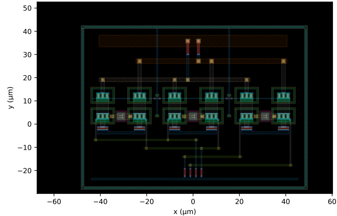
(d) co-design accepted point v3 (Alg. 1 through SpiceXplorer) 97.6 \times 70.5 \mu\text{m} = 6880 \mu\text{m}^2 S11 -10.05 / S22 -10.72 dB 190 mW
