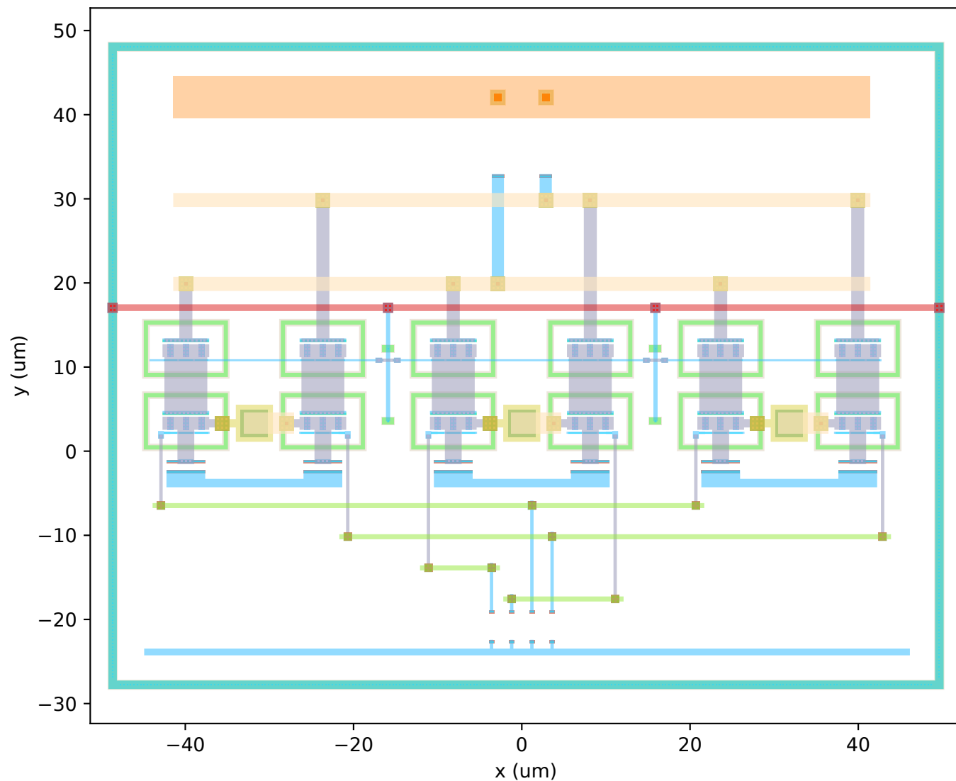
r1 best (run_22; r1 instrument, halo 8) S11 -10.04 dB S22 -10.76 dB MSB 8.21 dB LSB 2.23 dB BW 59.9 GHz swing 2.13 Vpp 173 mW 7664 \mu\text{m}^2
