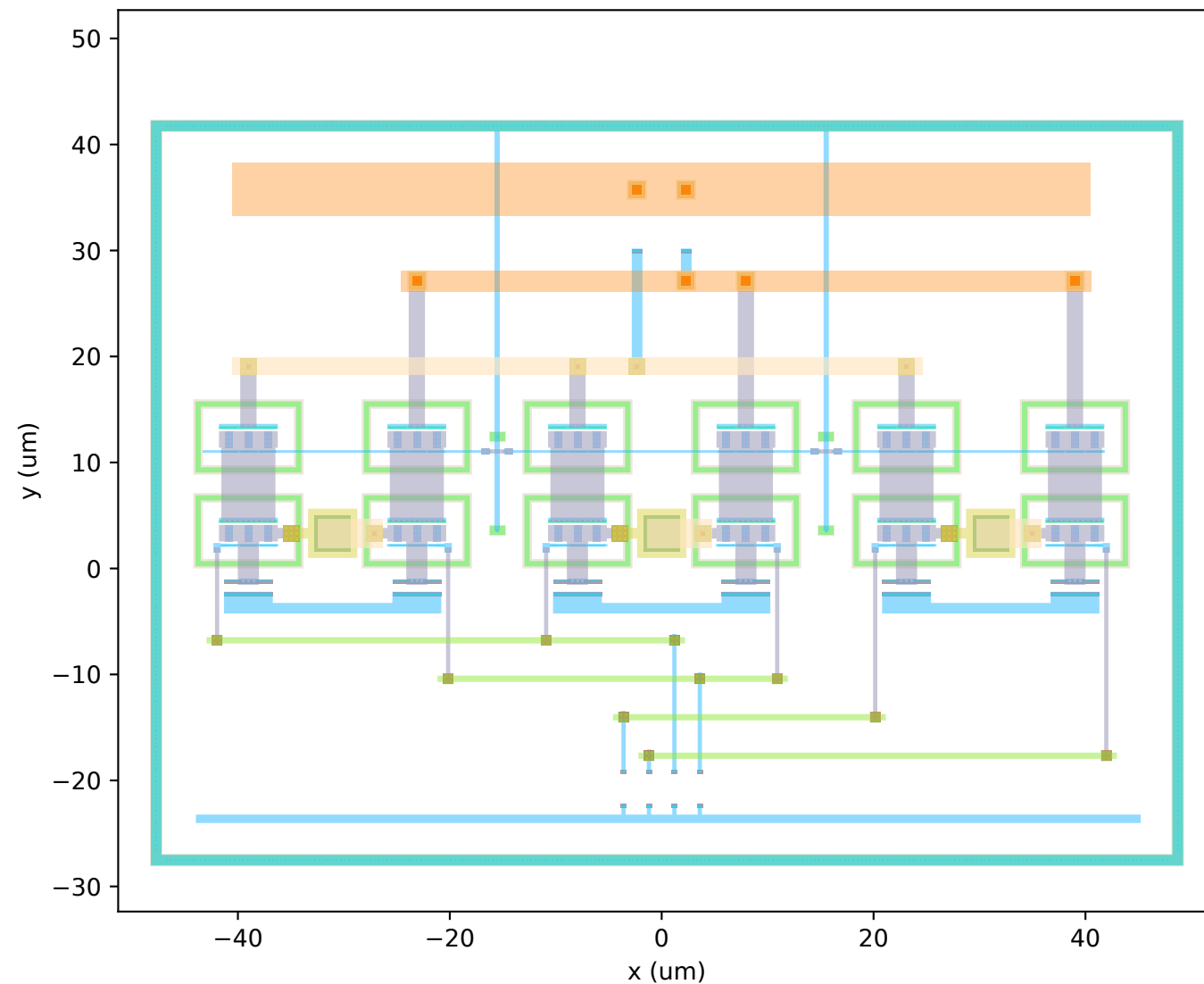
r2 accepted (island s3, run_38) S11 -10.07 dB S22 -10.79 dB MSB 8.20 dB LSB 2.23 dB BW 61.2 GHz swing 2.26 Vpp 190 mW 6880 \mu\text{m}^2
