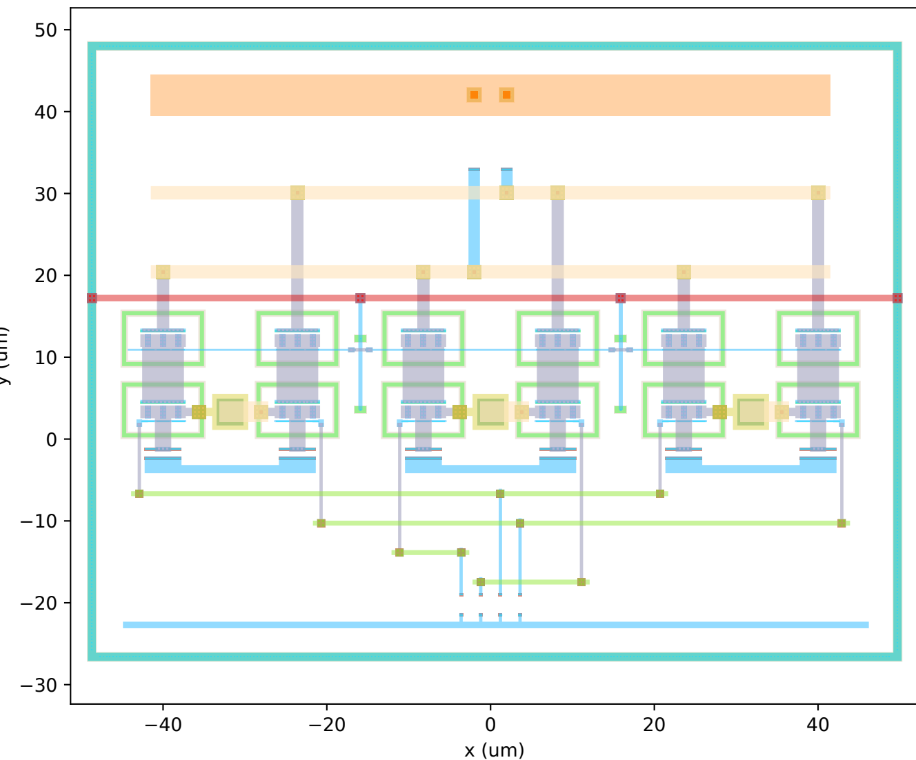
layout of record (r2 instrument) S11 -9.98 dB S22 -9.36 dB MSB 8.25 dB LSB 2.27 dB BW 59.2 GHz swing 2.21 Vpp 179 mW 7552 \mu\text{m}^2
