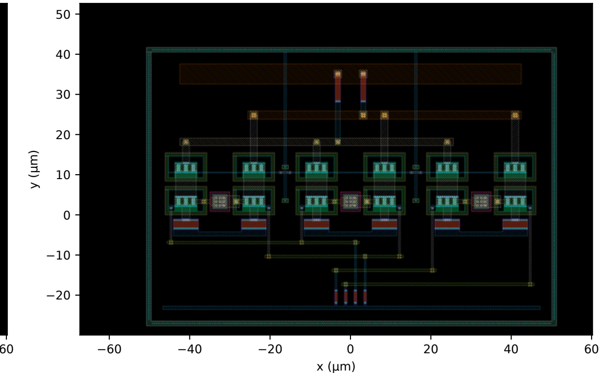
(e) co-design round 3 accepted point v4 (p/n balance objective) 102.0 \times 69.2 \mu\text{m} = 7055 \mu\text{m}^2 S11 -10.03 / S22 -10.71 dB 185 mW
