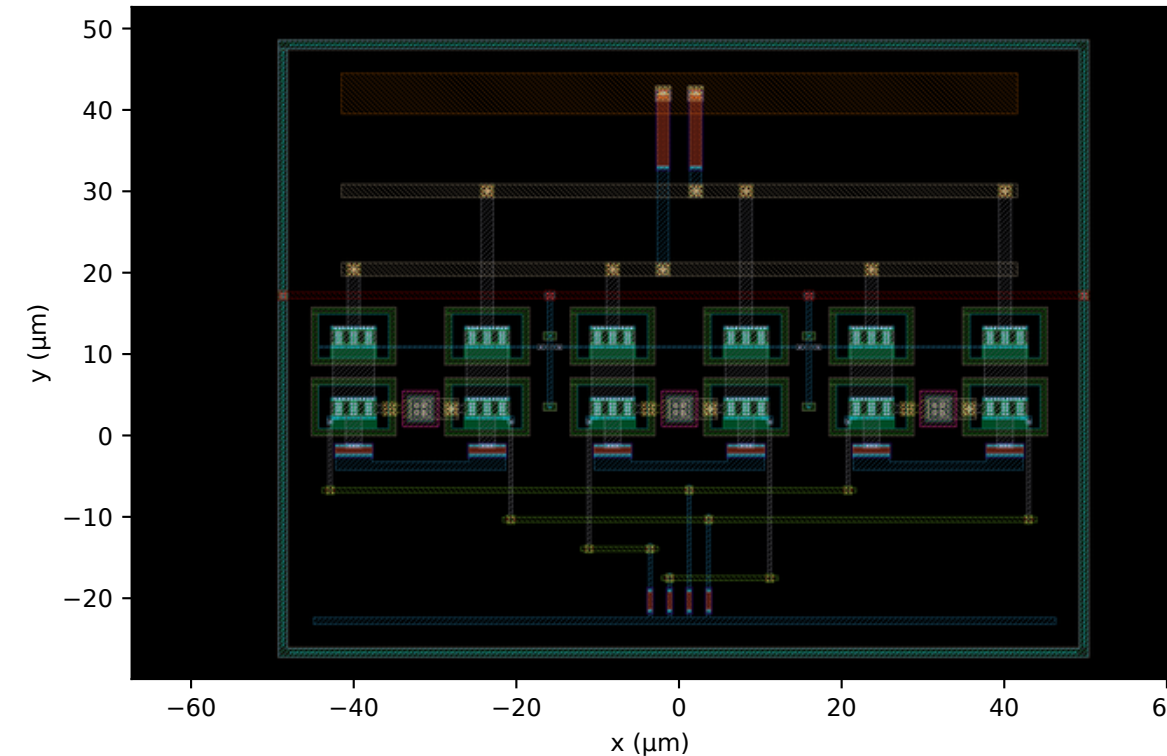
(c) layout of record v2 (block-local optimizer + RF review) 99.6 \times 75.8 \mu\text{m} = 7552 \mu\text{m}^2 S11 -9.94 / S22 -9.24 dB 179 mW
