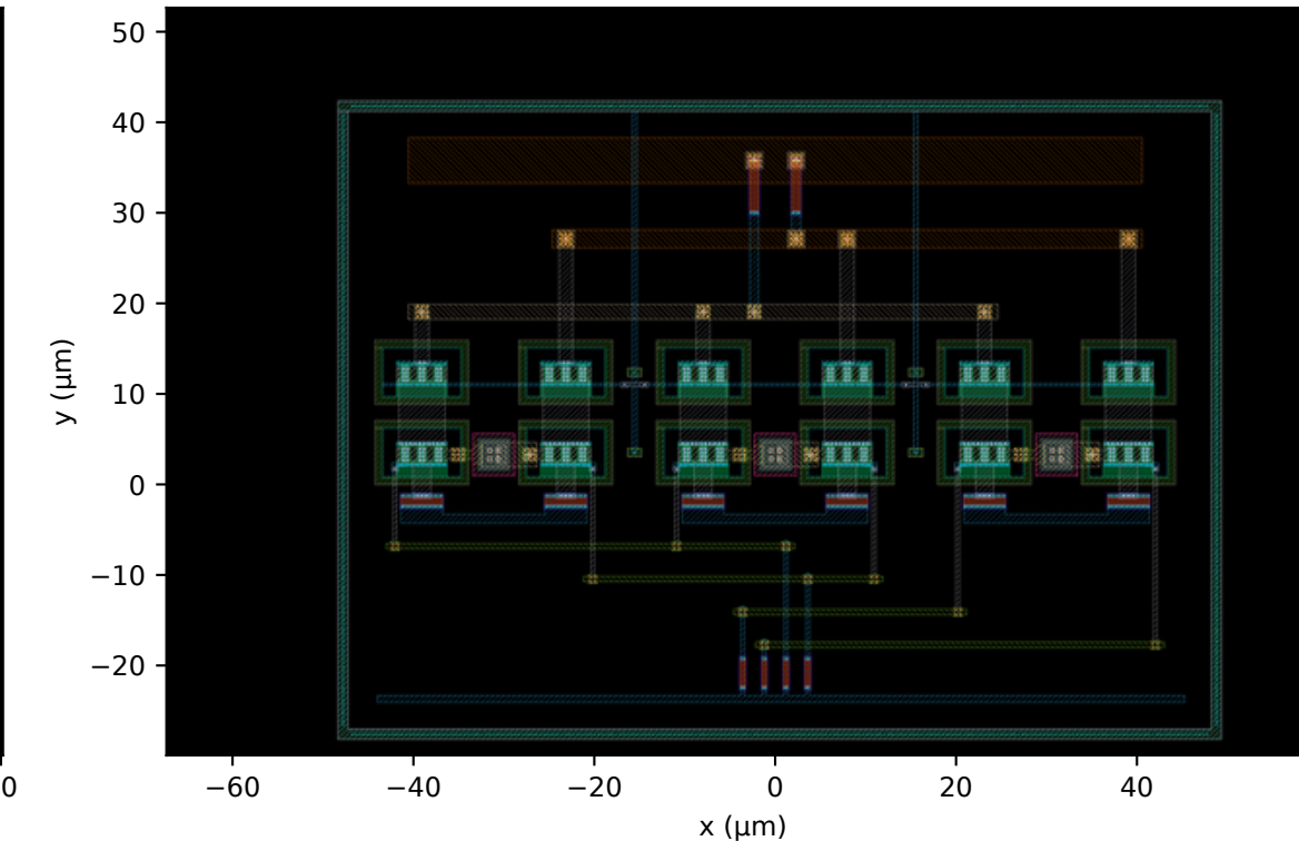
(d) co-design round 2, v3 (Alg. 1 through SpiceXplorer) 97.6 \times 70.5 \mu\text{m} = 6880 \mu\text{m}^2 S11 -10.05 / S22 -10.72 dB 190 mW
