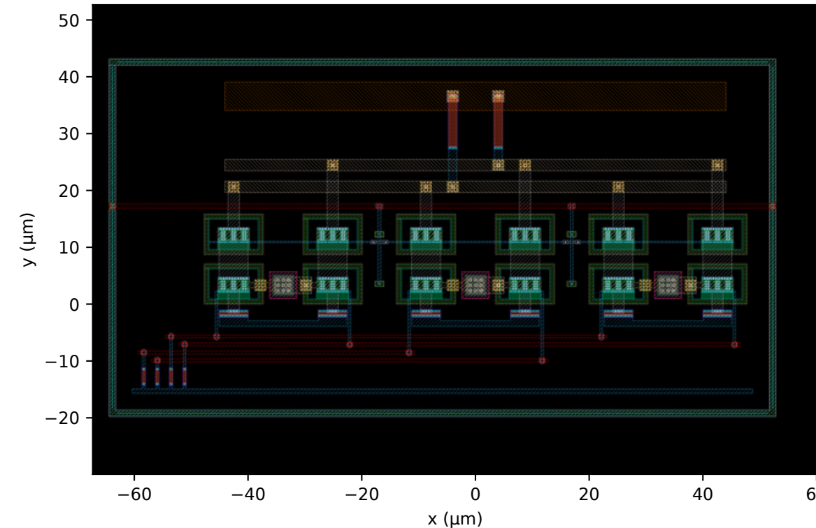
(b) first-pass layout (v1 floorplan, nominal sizing) 117.2 \times 62.9 \mu\text{m} = 7374 \mu\text{m}^2 S11 -8.90 / S22 -7.97 dB 191 mW
