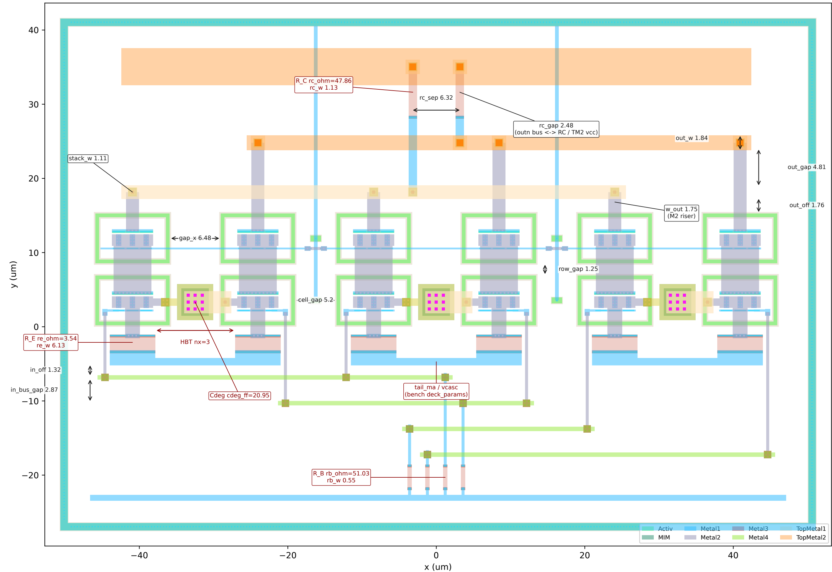
PAM-4 driver DAC — parameterized layout: black = layout knobs (um), red = electrical sizing that draws geometry, blue = structural options structural knobs: cell_order=1 (M0|M1|L0) bus_trim=1 out_split=1 sub_bus=1 c_strip=2 in_order=0
