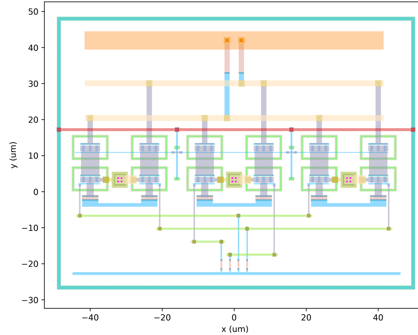
layout of record v2 (r2 instrument) S11 -9.98 dB S22 -9.36 dB MSB 8.25 dB LSB 2.27 dB BW 59.2 GHz swing 2.21 Vpp 179 mW 7552 \mu\text{m}^2
