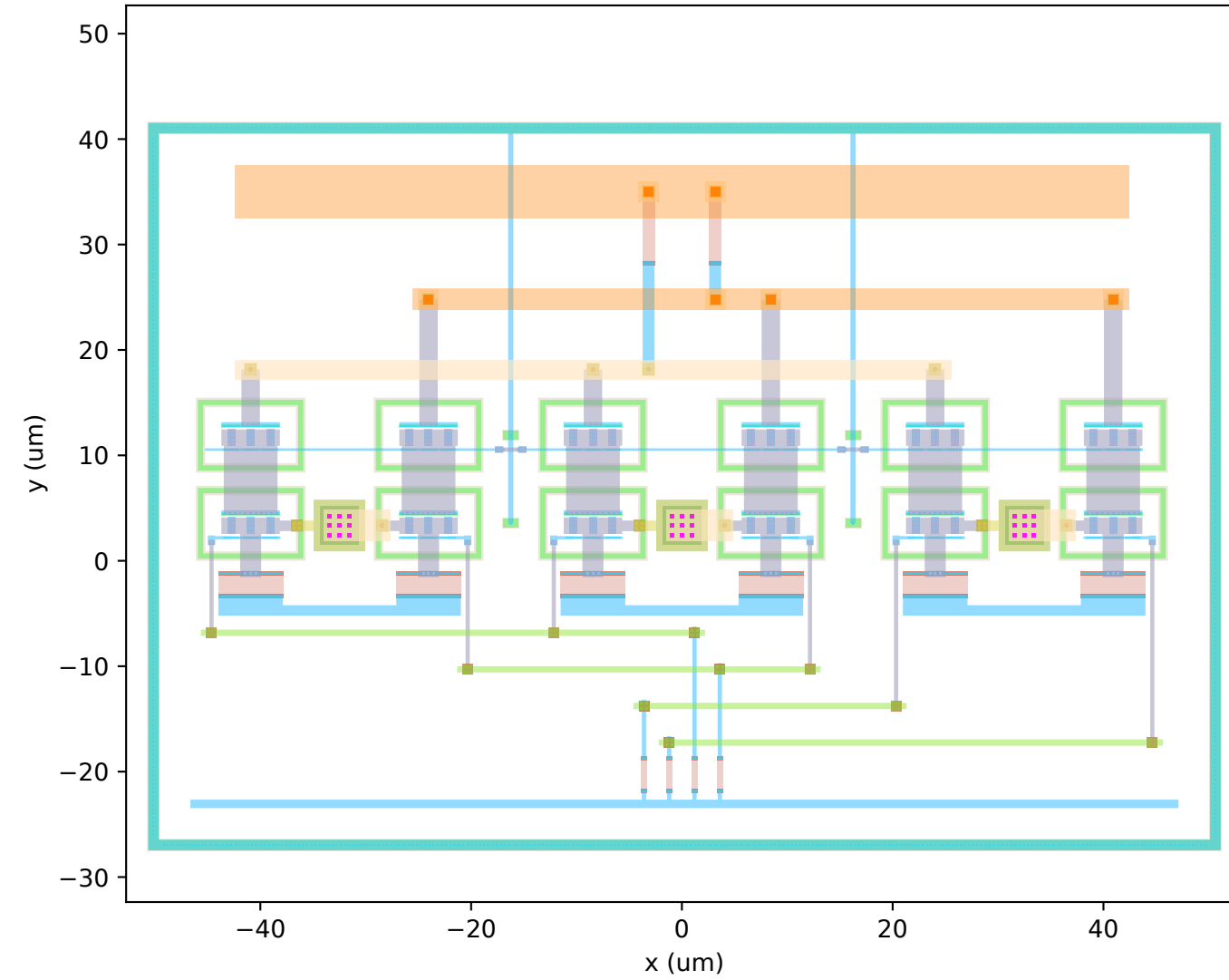
r3 accepted v4 (s23 run_30) S11 -10.07 dB S22 -10.81 dB MSB 8.24 dB LSB 2.27 dB BW 61.4 GHz swing 2.24 Vpp 185 mW 7055 \mu\text{m}^2
