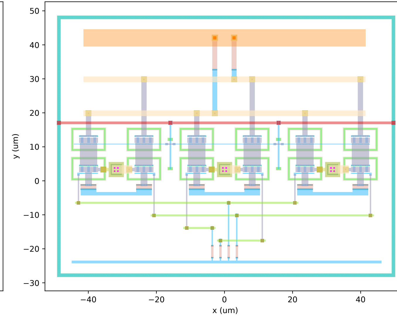
r1 best (run_22; r1 instrument, halo 8) S11 -10.04 dB S22 -10.76 dB MSB 8.21 dB LSB 2.23 dB BW 59.9 GHz swing 2.13 Vpp 173 mW 7664 \mu\text{m}^2
