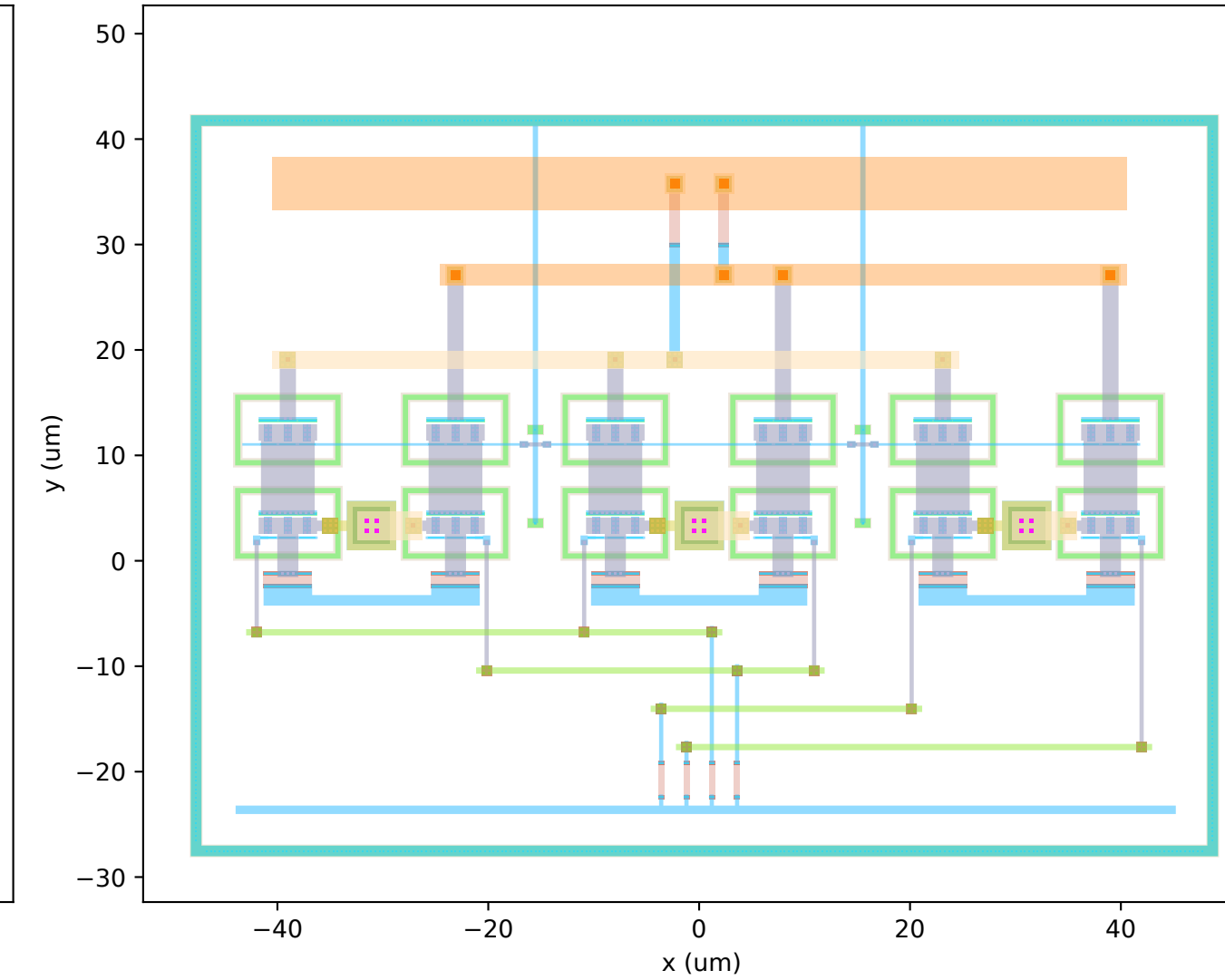
r2 accepted v3 (s3 run_38) S11 -10.07 dB S22 -10.79 dB MSB 8.20 dB LSB 2.23 dB BW 61.2 GHz swing 2.26 Vpp 190 mW 6880 \mu\text{m}^2
