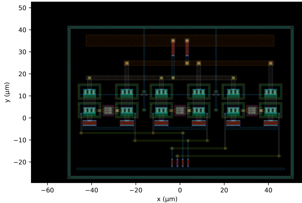
(e) co-design round 3 accepted point v4 (p/n balance objective) 102.0 \times 69.2 \mu\text{m} = 7055 \mu\text{m}^2 S_{11} -10.03 / S_{22} -10.71 dB 185 mW
