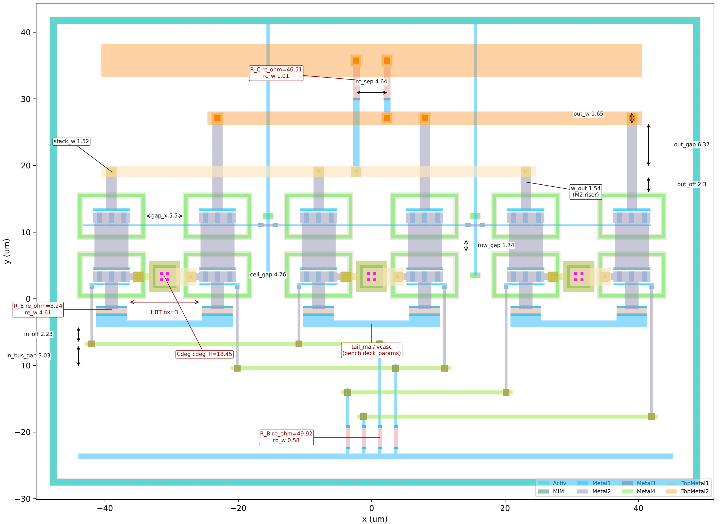
PAM-4 driver DAC — parameterized layout: black = layout knobs (um), red = electrical sizing that draws geometry, blue = structural options structural knobs: cell_order=1 (M0|M1|L0) bus_trim=1 out_split=1 sub_bus=1 c_strip=2
