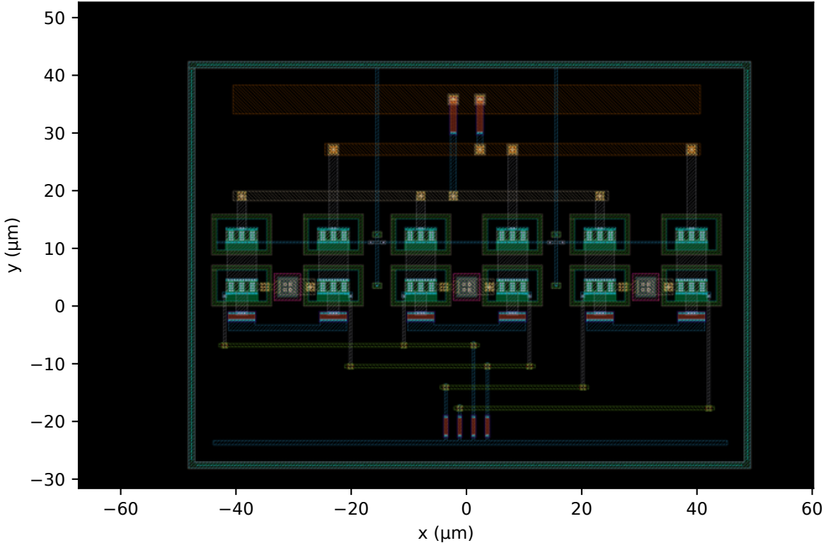
(d) co-design round 2, v3 (Alg. 1 through SpiceXplorer) 97.6 × 70.5 μm = 6880 μm 2 S11 -10.05 / S22 -10.72 dB 190 mW
