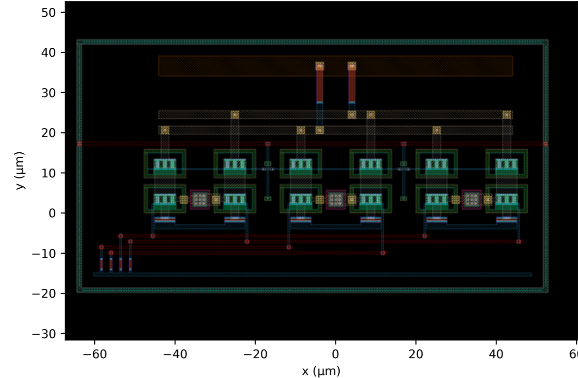
(b) first-pass layout (v1 floorplan, nominal sizing) 117.2 × 62.9 μm = 7374 μm 2 S11 -8.90 / S22 -7.97 dB 191 mW
