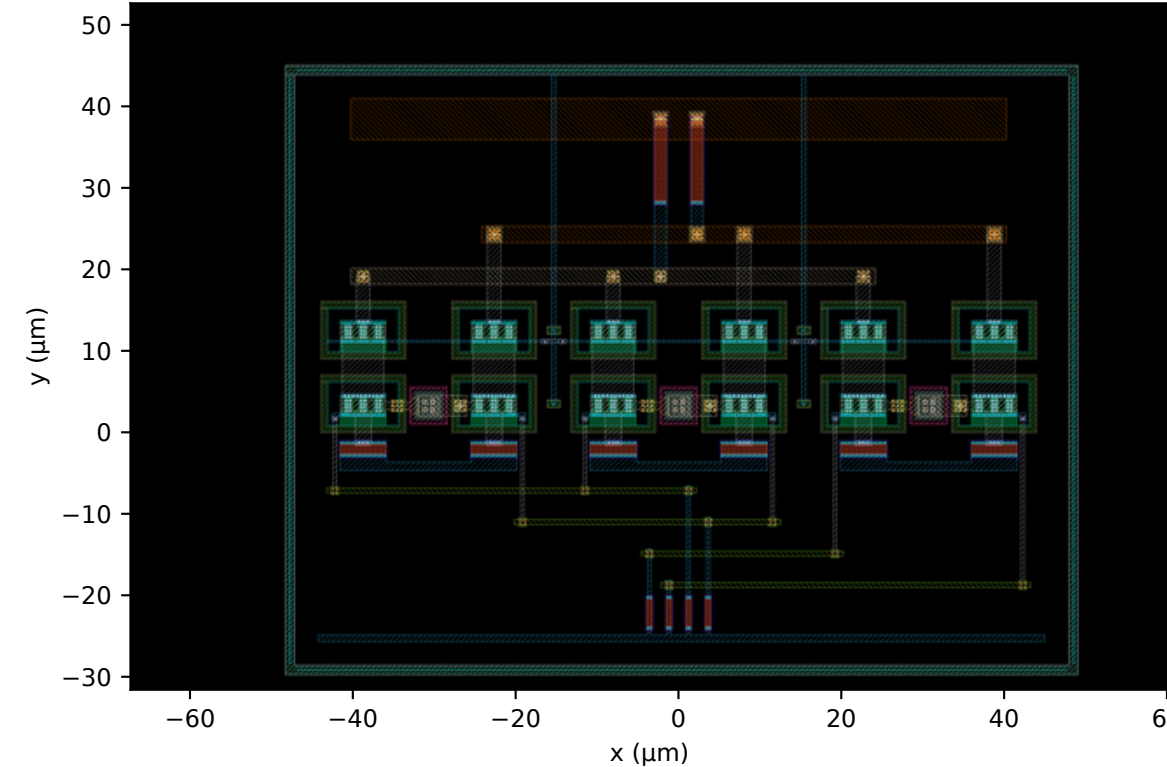
(f) co-design round 3 best-score point (r3_s12/run_26, the paper's design of record) 97.2 × 74.7 μm = 7268 μm 2 S11 -10.16 / S22 -10.28 dB 167 mW
