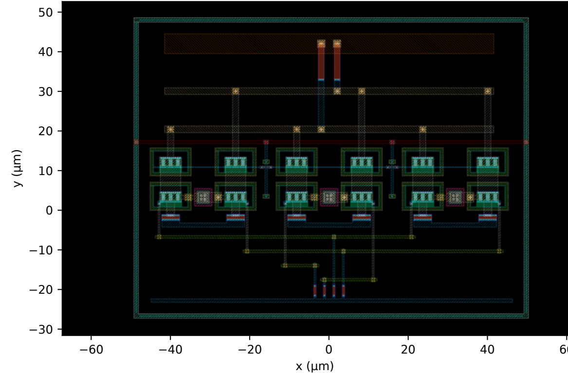
(c) layout of record v2 (block-local optimizer + RF review) 99.6 × 75.8 μm = 7552 μm 2 S11 -9.94 / S22 -9.24 dB 179 mW
