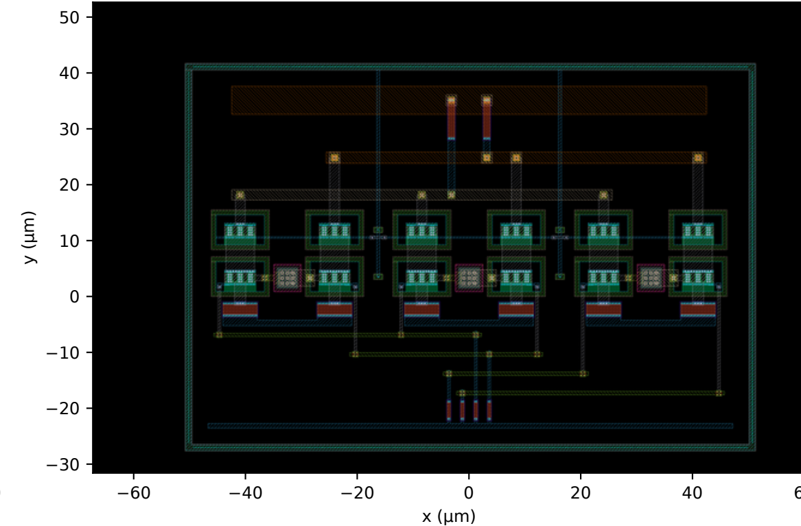
(e) co-design round 3 accepted point v4 (p/n balance objective) 102.0 × 69.2 μm = 7055 μm 2 S11 -10.03 / S22 -10.71 dB 185 mW
