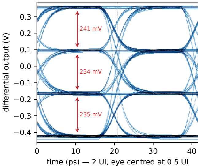
(g) round 4, co-designed RLM 0.996 swing 0.81\text{ V}_{pp}
