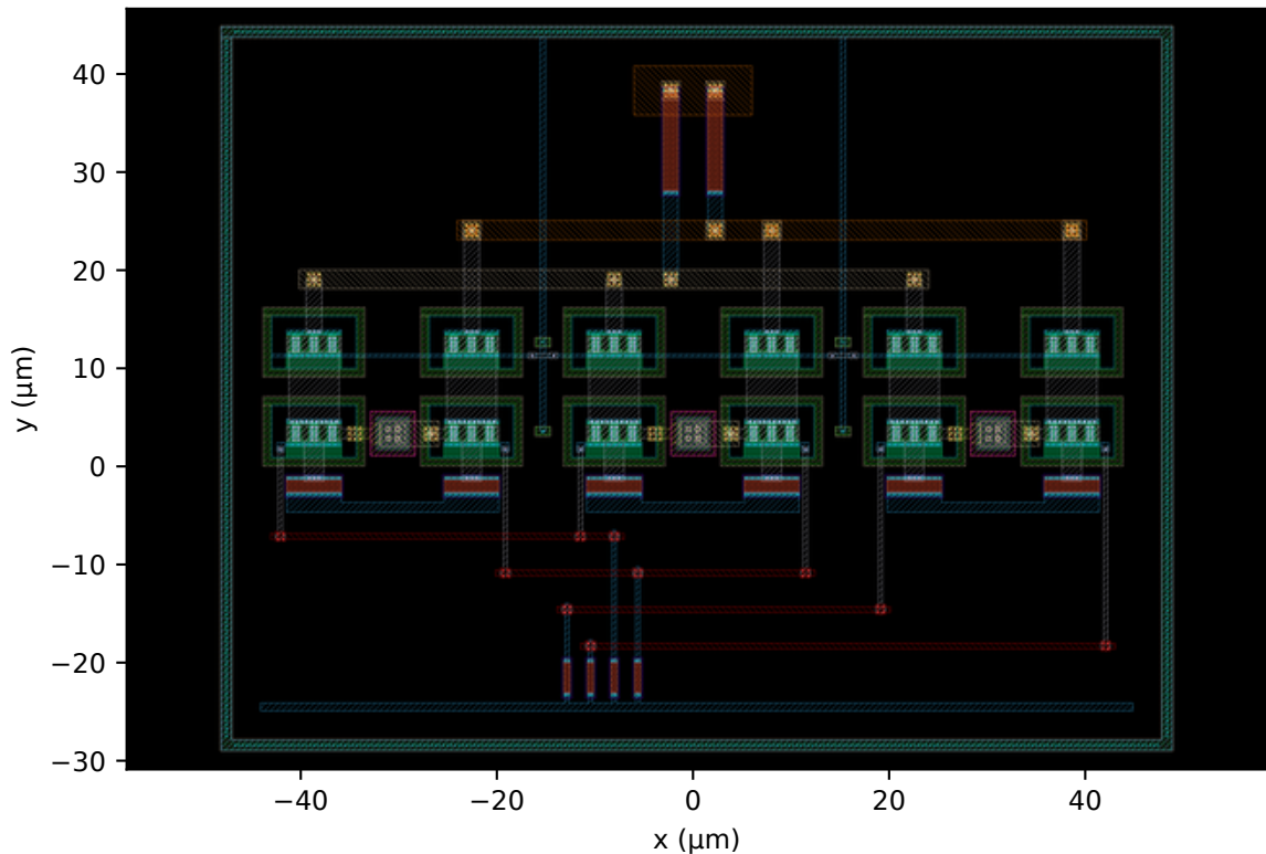
(g) co-design round 4 accepted point (r4_s10/run_29: reviewer-margin hinges + vcc_trim/rb_off opti 97.1 \times 73.8 \mu\text{m} = 7166 \mu\text{m}^2 S_{11} -10.24 / S_{22} -10.25 \text{ dB} 175 \text{ mW}
