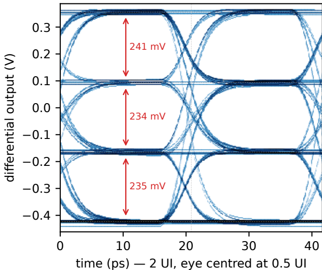
(g) round 4, co-designed RLM 0.996 swing 0.81 V_{pp}
