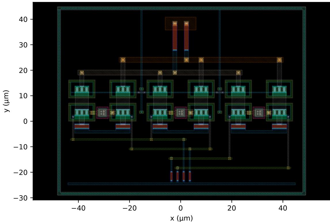
(g) co-design round 4 accepted point (r4_s10/run_29: reviewer-margin hinges + vcc_trim/rb_off opti 97.1 \times 73.8 \mu\text{m} = 7166 \mu\text{m}^2 S_{11} -10.17 / S_{22} -10.25 dB 175 mW
