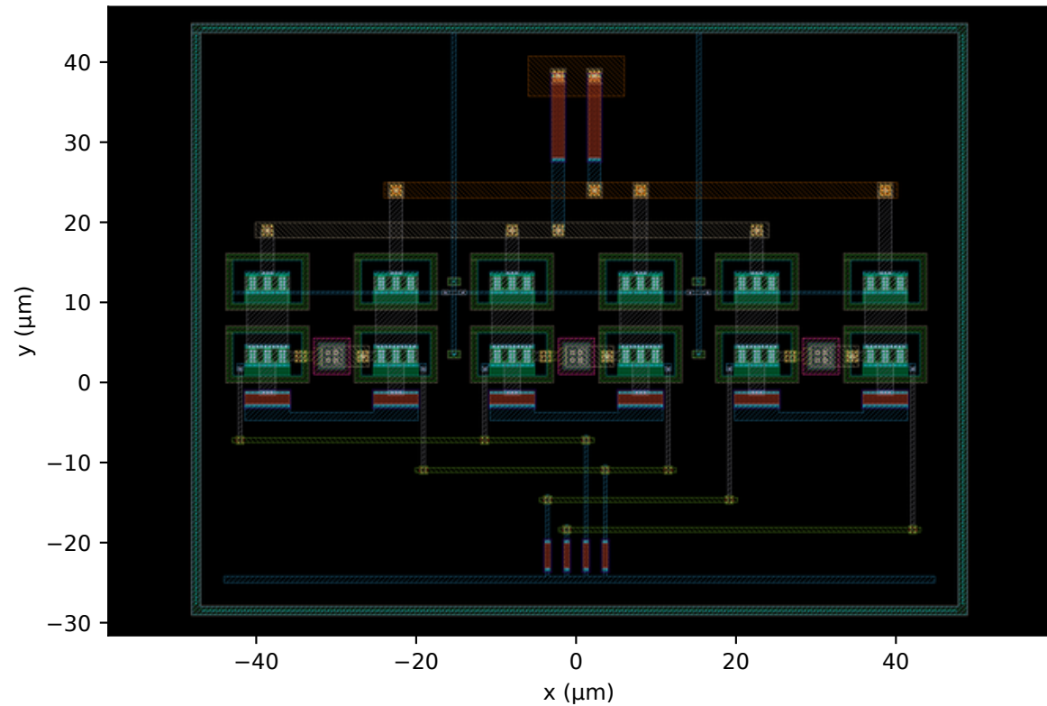
(g) co-design round 4 accepted point (r4_s10/run_29: reviewer-margin hinges + vcc_trim/rb_off option) 97.1 \times 73.8 \mu\text{m} = 7166 \mu\text{m}^2 S11 -10.17 / S22 -10.25 dB 175 mW
