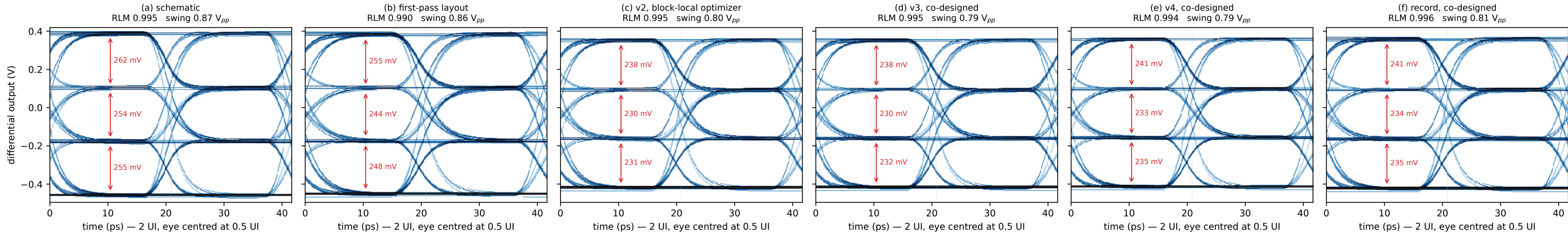
48 GBd PAM-4 eye — 200 mV pp input, 4 ps edges, seed-7 MSB/LSB streams; post-layout tiers on the kpex 2.5D CC extraction
