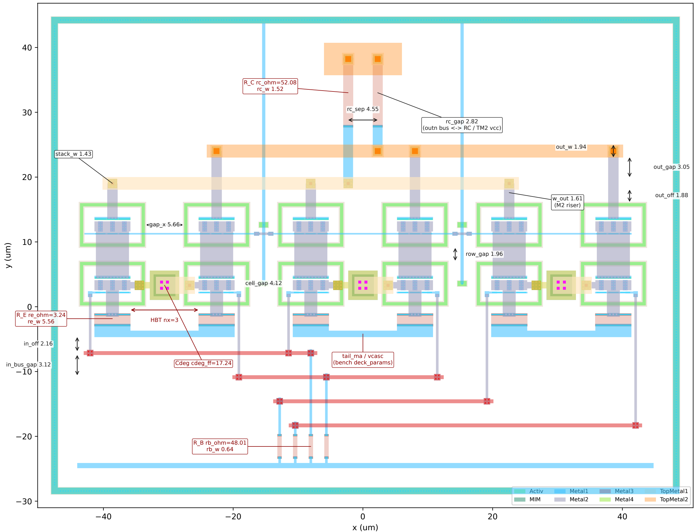
PAM-4 driver DAC — parameterized layout: black = layout knobs (um), red = electrical sizing that draws geometry, blue = structural options structural knobs: cell_order=1 (M0|M1|L0) bus_trim=1 out_split=1 sub_bus=1 c_strip=2 in_order=0
