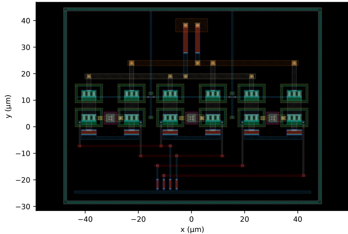
(g) co-design round 4 accepted point (r4_s10/run_29: reviewer-margin hinges + vcc_trim/rb_off option) 97.1 \times 73.8 \mu\text{m} = 7166 \mu\text{m}^2 S11 -10.24 / S22 -10.25 dB 175 mW
