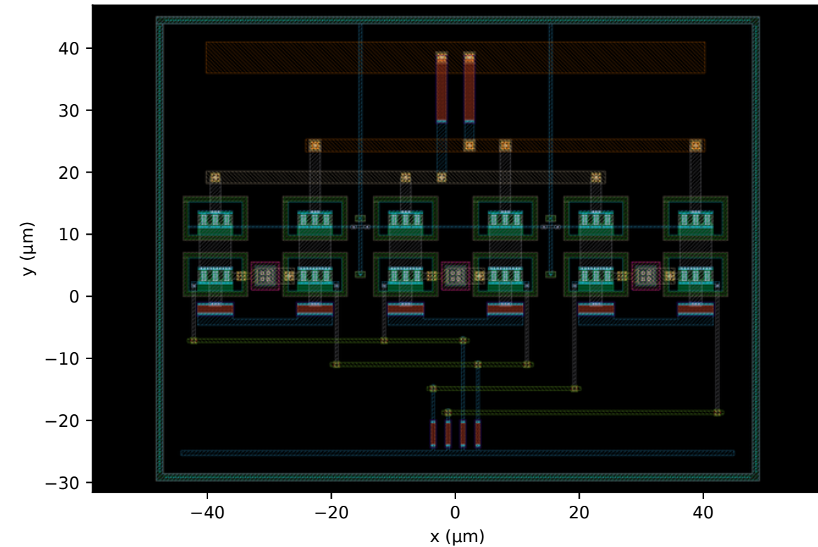
(f) co-design round 3 best-score point (r3_s12/run_26, the paper's design of record) 97.2 \times 74.7 \mu\text{m} = 7268 \mu\text{m}^2 S11 -10.16 / S22 -10.28 dB 167 mW
