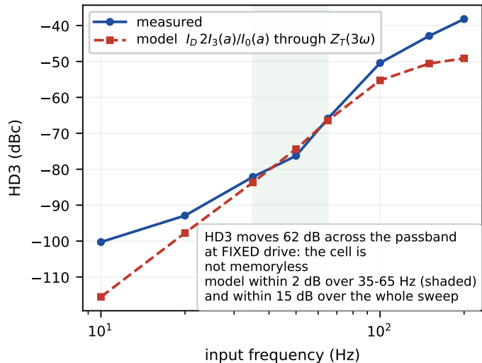
(b) HD3 vs frequency at 43.75 mVpp
