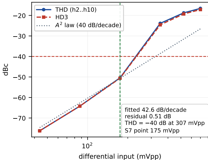
(a) distortion vs amplitude, f_{in} = 50 Hz
