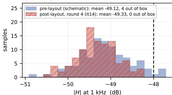
spec: stopband \leq -48 dB
