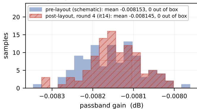
spec: |\text{gain}| \leq 0.2 dB
