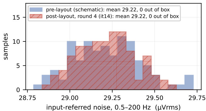
spec: noise < 40 \mu Vrms
