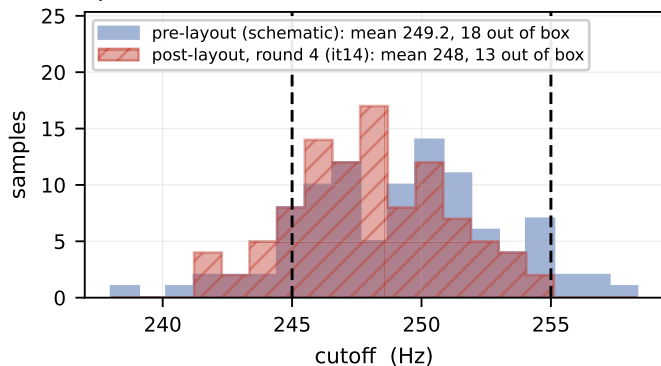
spec: in band 245–255 Hz
