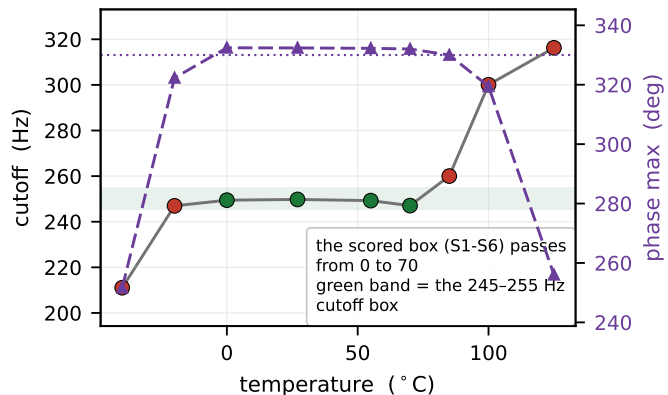
(d) full grid — 16 of 45 pass the scored box
