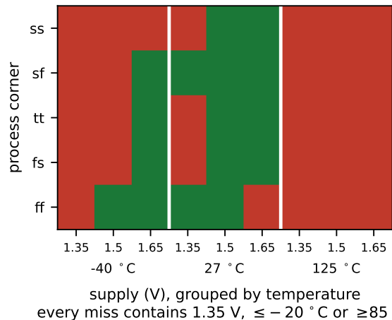
(d) full grid — 16 of 45 pass the scored box
