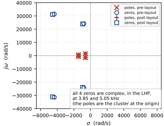
(c) full plane: poles and zeros
