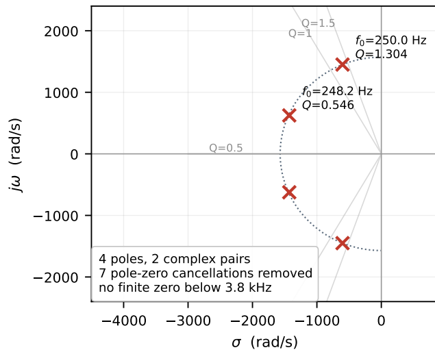
(b) post-layout (extracted C)
