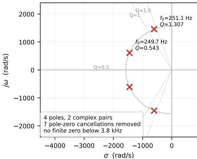
(a) pre-layout
