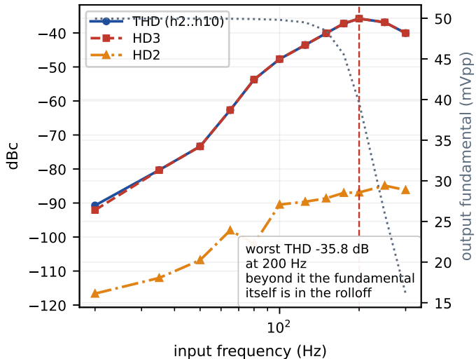
(a) extracted cell, 50 mVpp
