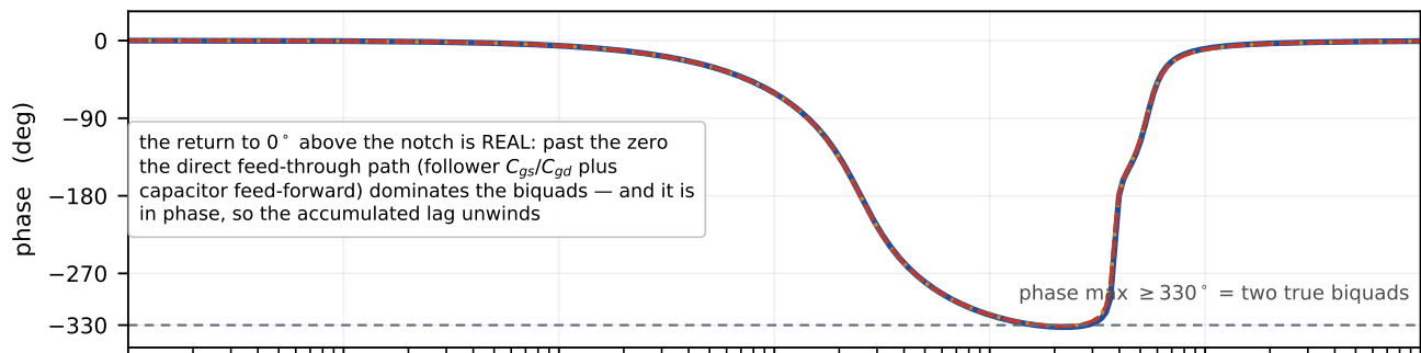
(c) after layout — before: the 3-5 kHz spike is the notch region, not a resonance
