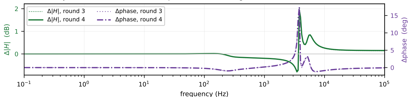
(c) after layout — before: the 3-5 kHz spike is the notch region, not a resonance
