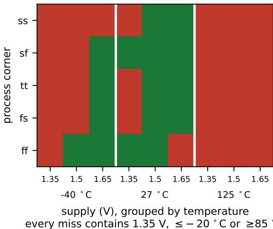
(d) full grid — 16 of 45 corners pass every line
