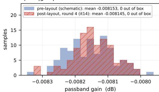
spec: |\text{gain}| \leq 0.2 dB
