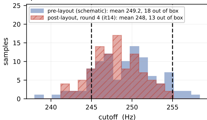
spec: in band 245–255 Hz
