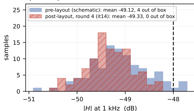
spec: stopband \leq -48 dB
