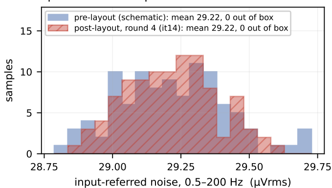
spec: noise < 40 \mu Vrms
