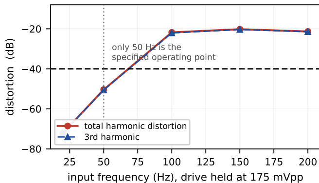
(c) sweep over input frequency
