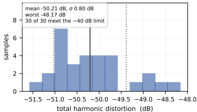
(b) mismatch Monte Carlo, 30 draws
