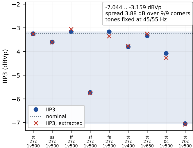
(a) IIP3 over the certified axes
