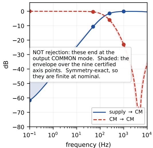
(c) nominal common-mode paths
