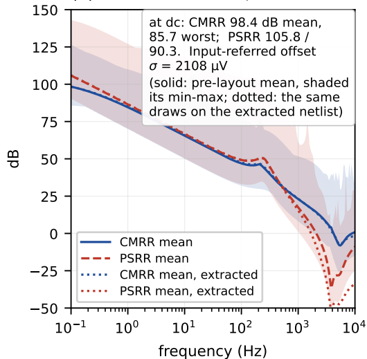
(b) mismatch-limited, 1024 draws
