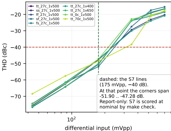
(a) the ladder at every corner, f_{in} = 50 Hz
