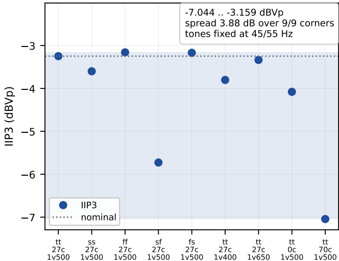
(a) IIP3 over the certified axes
