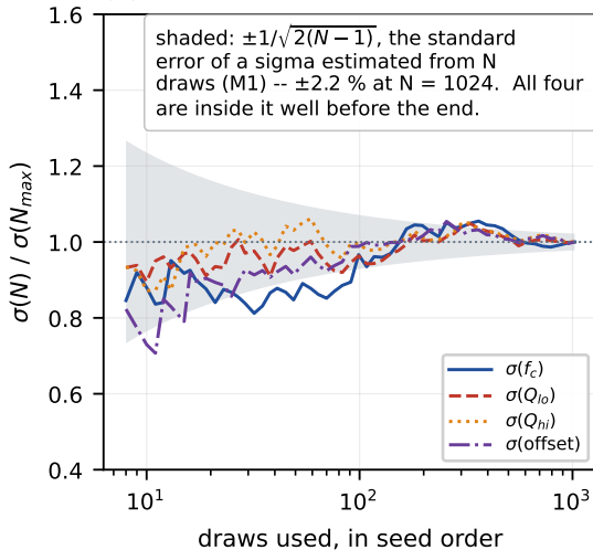
(a) extraction MC
