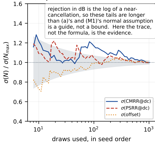
(b) rejection MC
