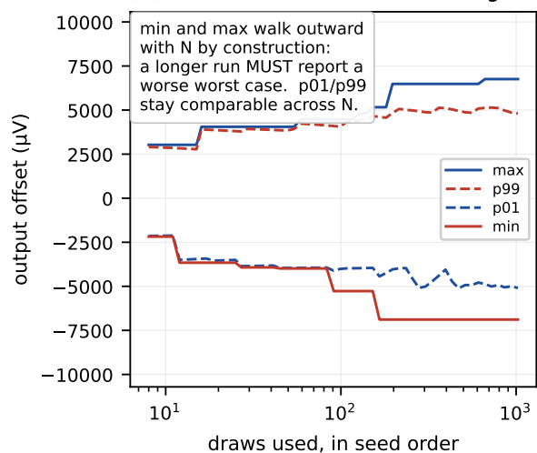
(c) order statistics do not converge
