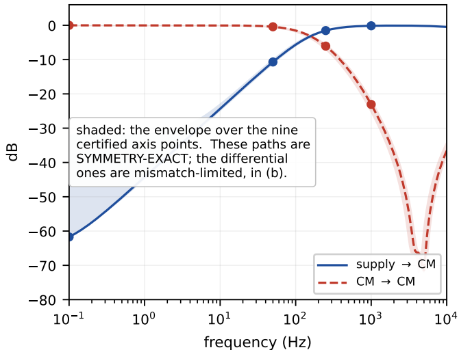
(a) nominal common-mode paths
