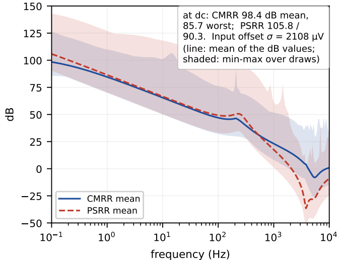
(b) mismatch-limited, 1024 draws
