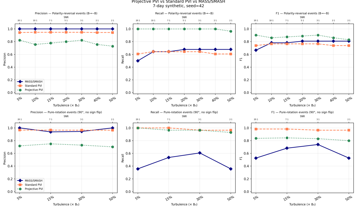
Figure 5: Tandem comparison of MASS/SMASH, standard PVI, and projective PVI (pPVI) across turbulence levels. Top row: polarity-reversal benchmark (B → -B transitions). MASS/SMASH: P = 1.000 throughout; pPVI: R \approx 1.000 throughout; standard PVI: intermediate. Bottom row: pure-rotation benchmark (90° direction change, no sign flip). MASS/SMASH recall peaks at 61% (30% turbulence) then falls back to 36% (50% turbulence) because the MDL gain for 90° rotations is \sim 4\times lower than for sign flips; pPVI and standard PVI maintain R \geq 0.929 .
