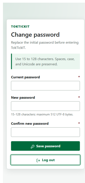
Figure: Mandatory password change at mobile width - artifacts/lab-03/screenshots/authentication/mandatory-change-mobile.png
