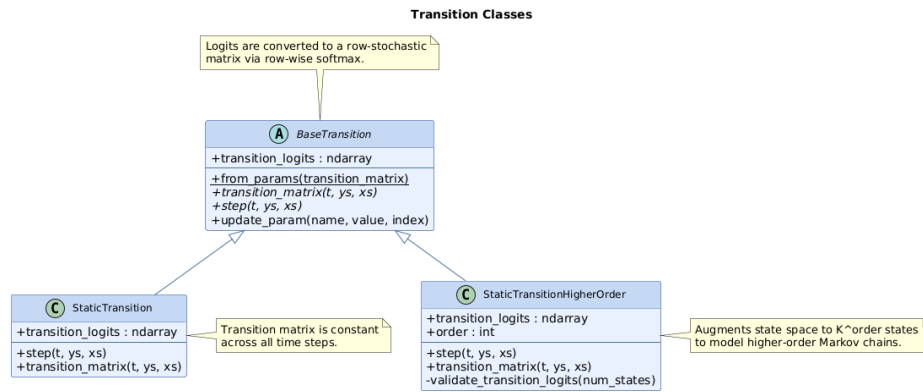
Figure 7: Transition class hierarchy. Both implementations store parameters as logits and convert them to a row-stochastic matrix via row-wise softmax. StaticTransition uses a constant K \times K matrix, while StaticTransitionHigherOrder augments the state space to K^{\text{order}} states to represent a higher-order Markov chain.
