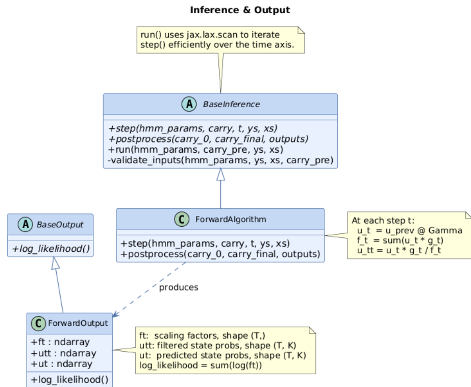
Figure 8: Inference and output class hierarchy. BaseInference.run() iterates step() across the time axis using jax.lax.scan . ForwardAlgorithm implements the forward filtering pass and produces a ForwardOutput storing the scaling factors f_t , filtered state probabilities u_{t|t} , and predicted state probabilities u_t . The log-likelihood is computed as \sum_t \log f_t .
