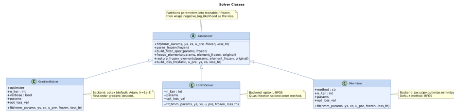
Figure 9: Solver class hierarchy. BaseSolver partitions parameters into trainable and frozen subsets and wraps the negative log-likelihood as the loss function. The three concrete solvers share the same interface but differ in their optimization backend: GradientSolver uses first-order gradient descent via optax , LBFGSSolver uses quasi-Newton L-BFGS via optax , and Minimizer wraps jax.scipy.optimize.minimize .
