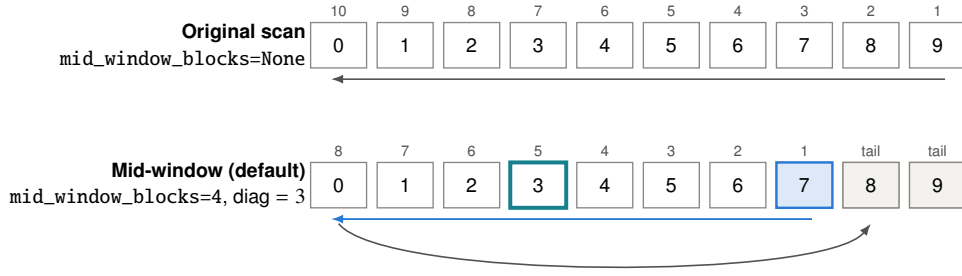
Figure 3. Key-block visiting order for a query tile whose diagonal block is 3, with 10 key blocks. Small numbers give the visiting position. The default mid-window order starts at j_0 = \min(3 + 4, 9) = 7 (blue), sweeps 7 \rightarrow 0 past the diagonal block (teal outline), then visits the tail blocks 8 and 9. Every block is visited in both orders; only the order changes.
