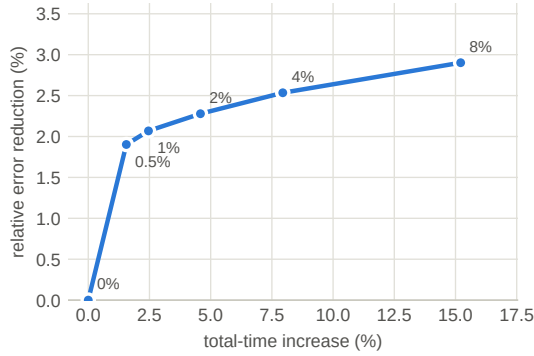
Figure 5. Cost and benefit of V residual repair (labels are budgets). Most of the error reduction comes from the first 0.5% of tokens; larger budgets trade more time for smaller additional gains.
