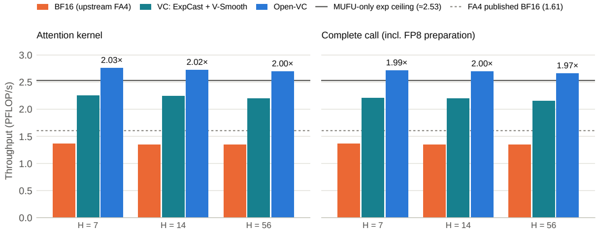
Figure 4. Attention throughput (FLOP model 4S^2HD ) of BF16, VC and Open-VC on the captured activations. Labels give Open-VC’s speedup over BF16. Solid line: the approximate B200 ceiling for a kernel that evaluates every exponential on MUFU (Table 1). Dotted line: FA4’s published B200 BF16 throughput [16].
