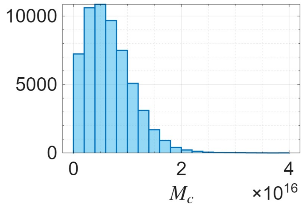
NGC3726 ( R_{\text{max}} = 32.52\text{kpc} )
