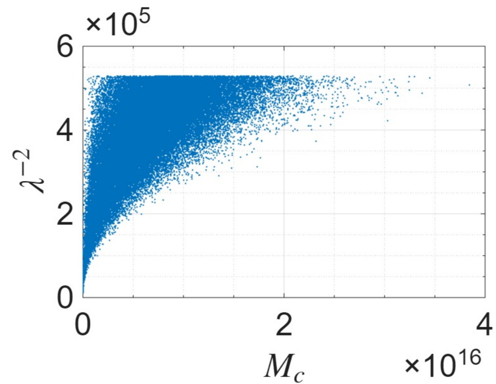
NGC3726 ( R_{\text{max}} = 32.52\text{kpc} )
