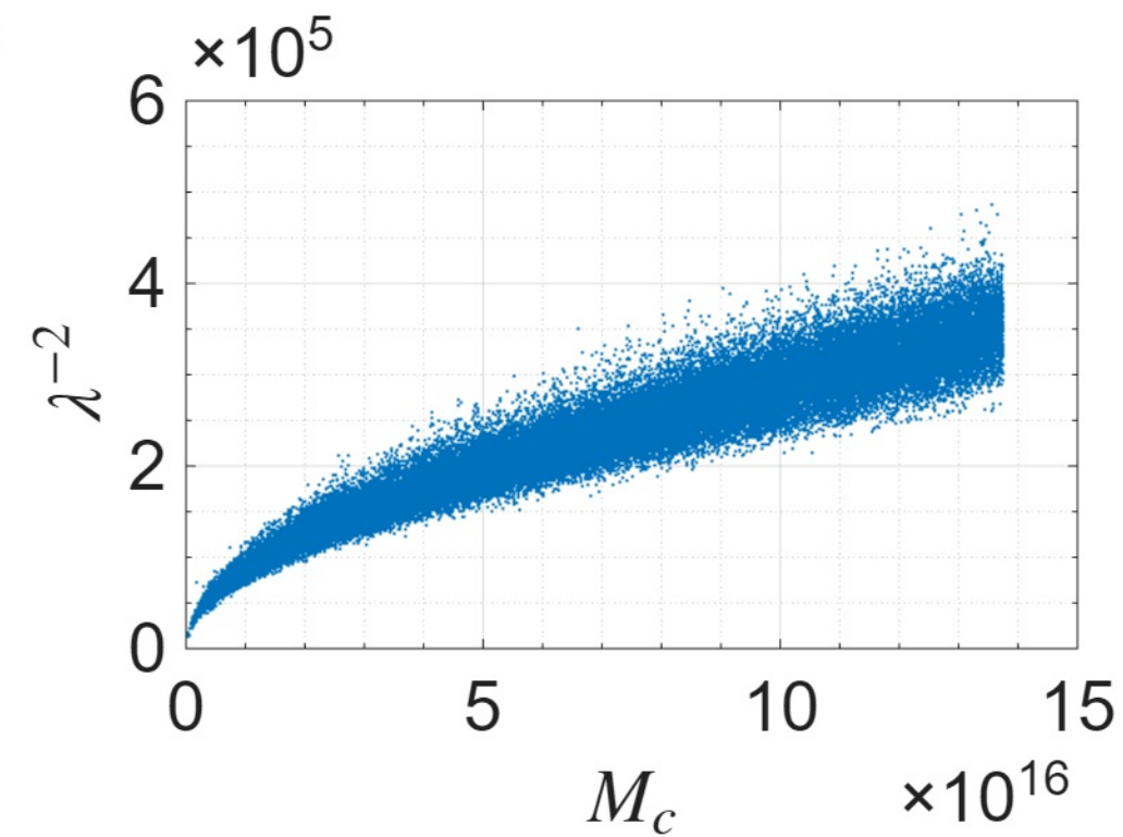
NGC3769 ( R_{\text{max}} = 37.16\text{kpc} )
