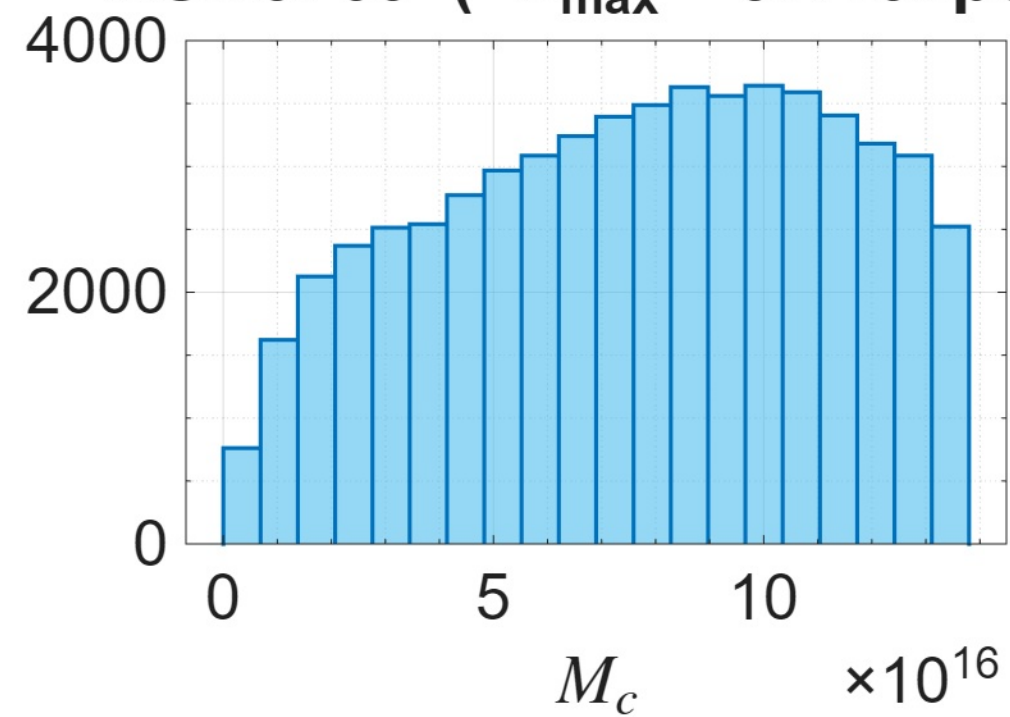
NGC3769 ( R_{\text{max}} = 37.16\text{kpc} )
