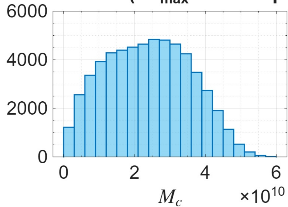
NGC3877 ( R_{\text{max}} = 11.35\text{kpc} )
