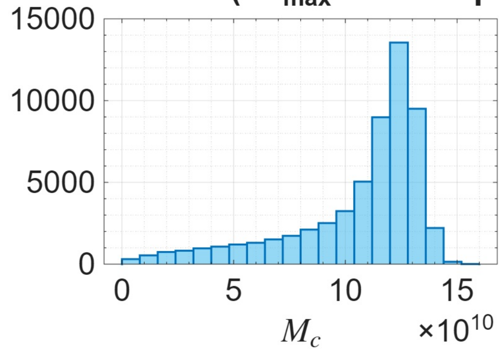
NGC3953 ( R_{\text{max}} = 15.68\text{kpc} )
