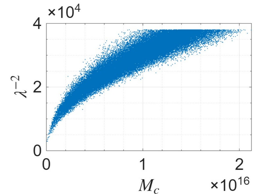
NGC3972 ( R_{\text{max}} = 8.72\text{kpc} )
