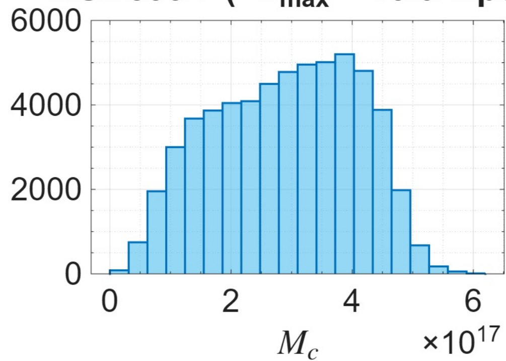
NGC3992 ( R_{\text{max}} = 46.02\text{kpc} )
