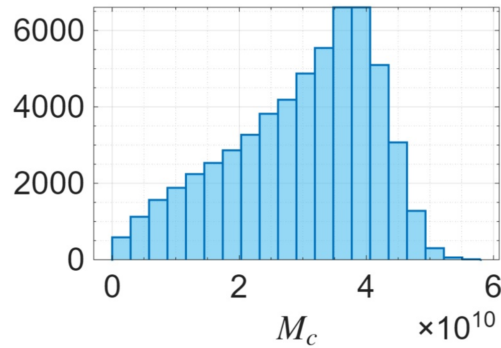
NGC4051 ( R_{\text{max}} = 12.19\text{kpc} )
