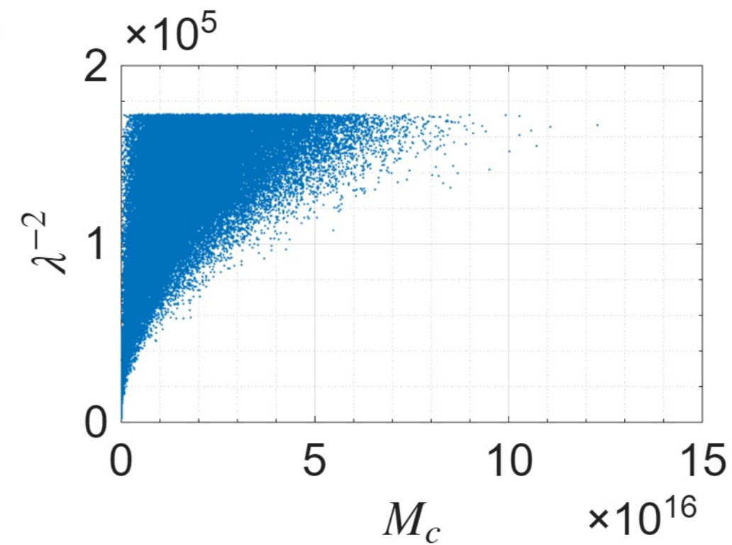
NGC4138 ( R_{\text{max}} = 18.58\text{kpc} )
