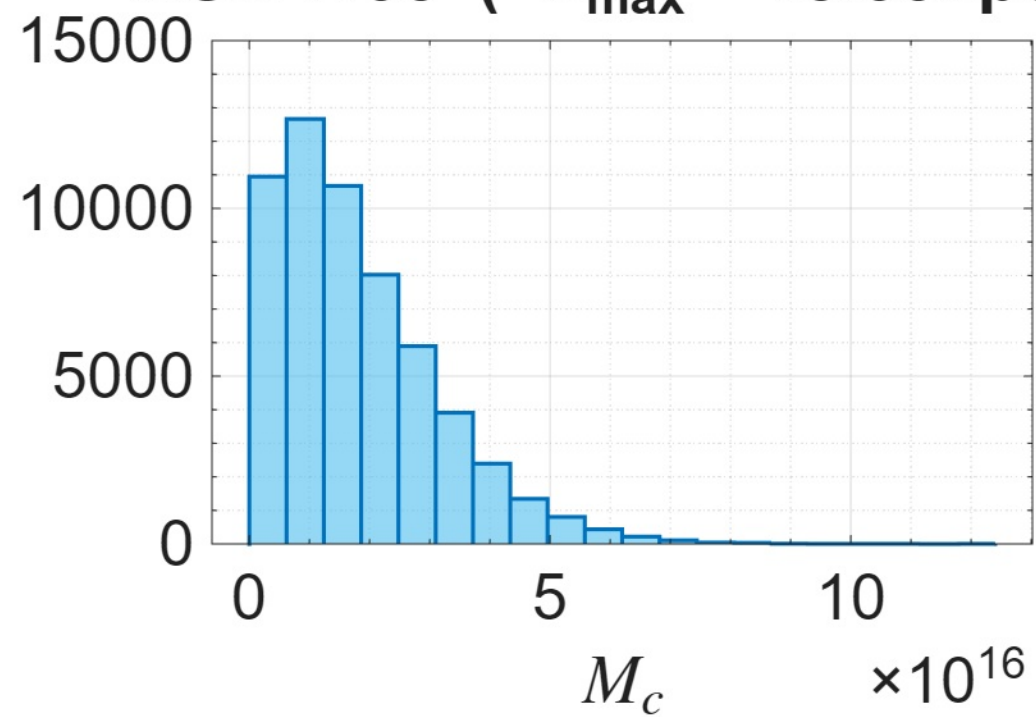
NGC4138 ( R_{\text{max}} = 18.58\text{kpc} )
