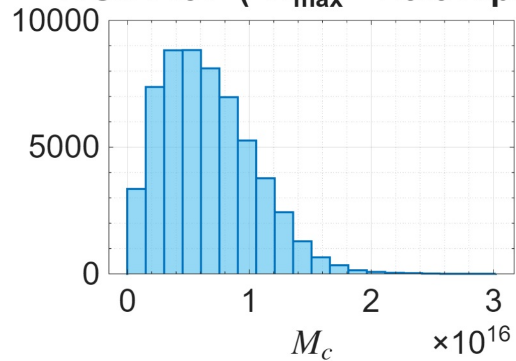
NGC4157 ( R_{\text{max}} = 29.61\text{kpc} )
