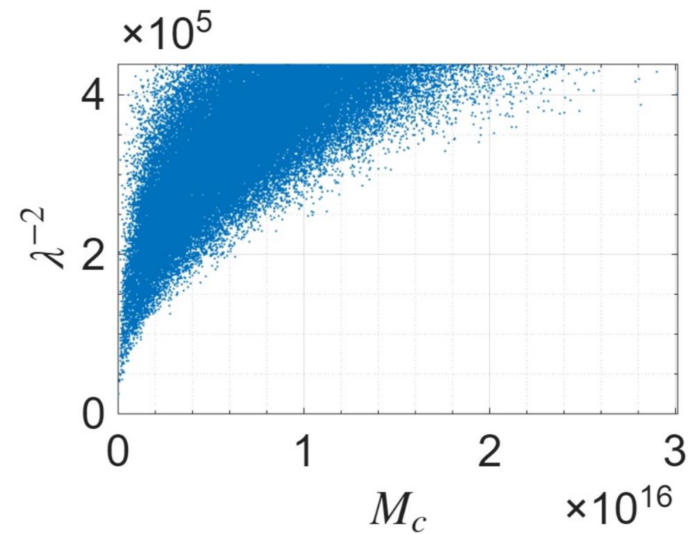
NGC4157 ( R_{\text{max}} = 29.61\text{kpc} )
