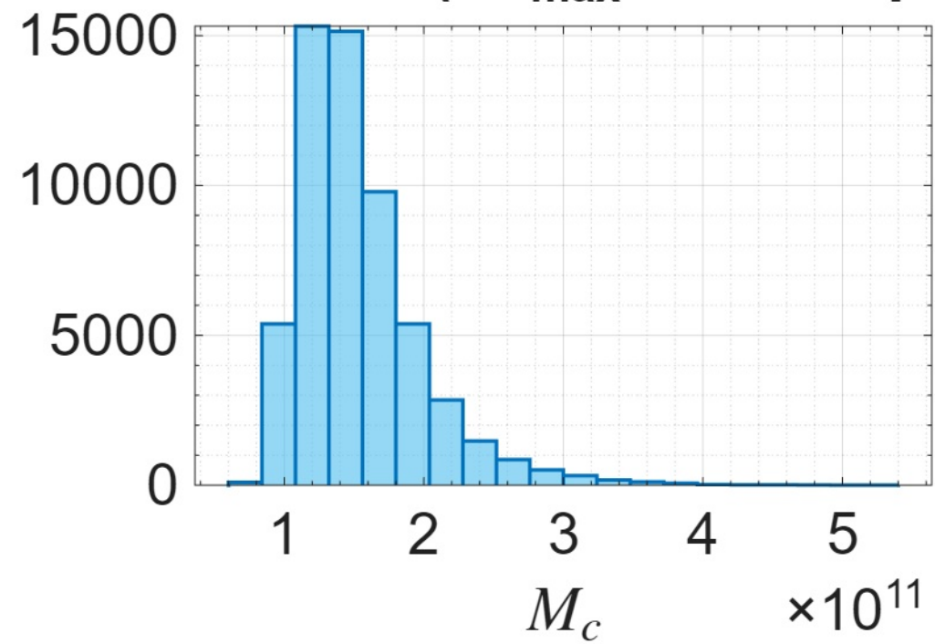
NGC4183 ( R_{\text{max}} = 21.02\text{kpc} )
