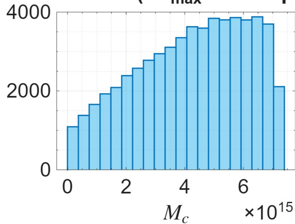
NGC4214 ( R_{\text{max}} = 5.63\text{kpc} )
