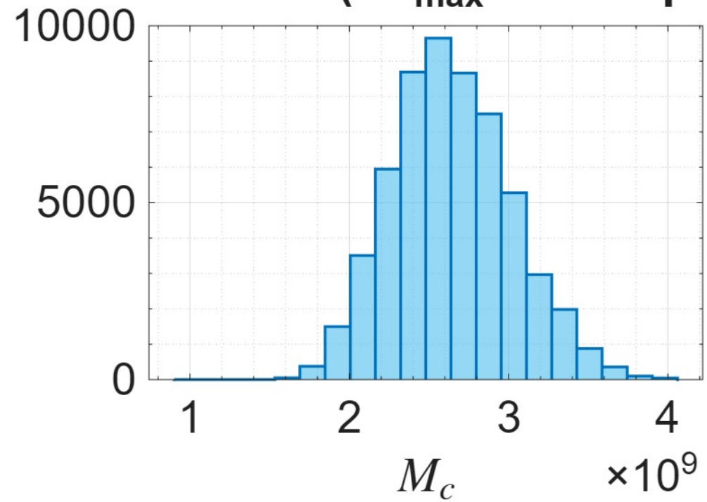
NGC4389 ( R_{\text{max}} = 5.32\text{kpc} )
