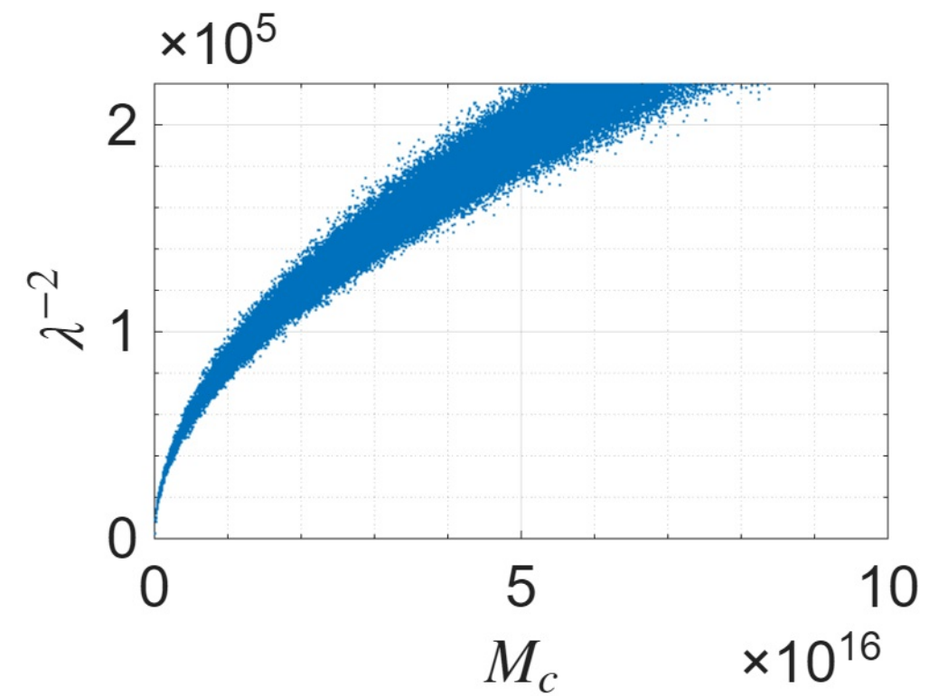
NGC4559 ( R_{\text{max}} = 20.97\text{kpc} )
